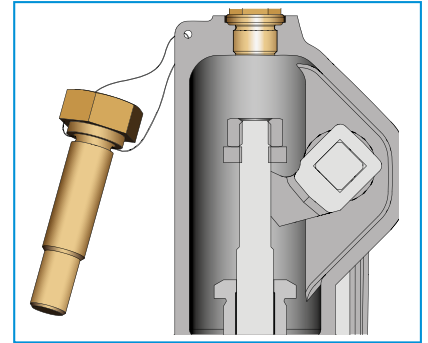
B Test gag: Blocking of the safety valve for pressure testing the pressure system.
