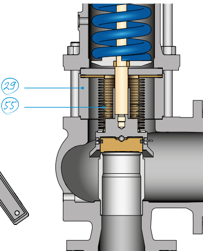
Bellows design Si 4402
