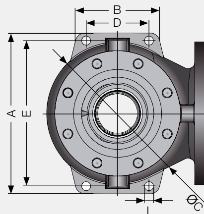
Support brackets
