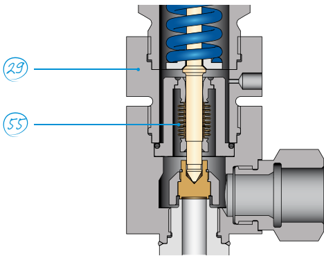
Bellows design Si 0429
